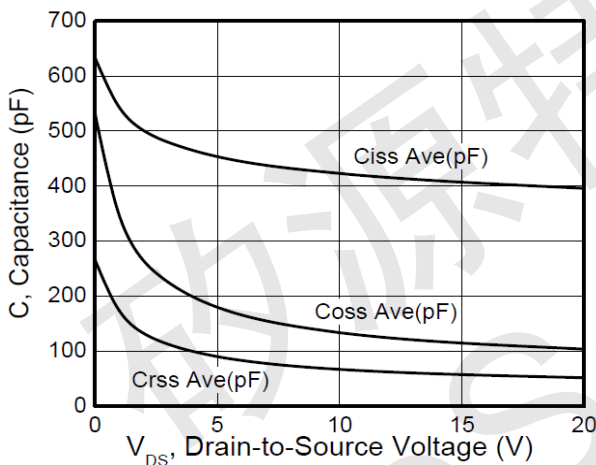
Figure 3. Capacitance
