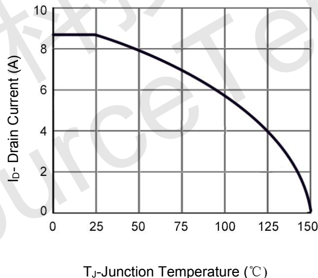
Figure 4 Drain Current
