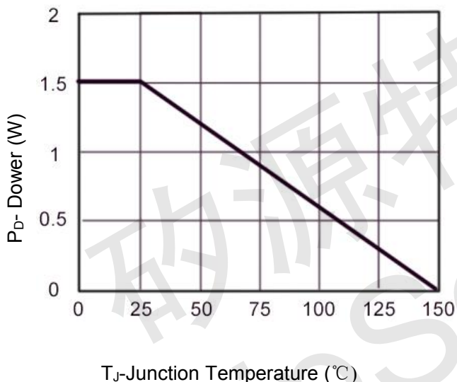
Figure 3 Power Dissipation
