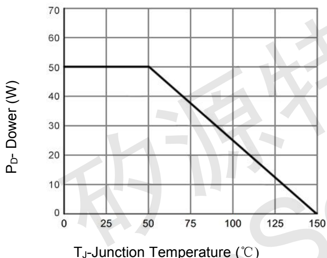
Figure 3 Power De-rating
