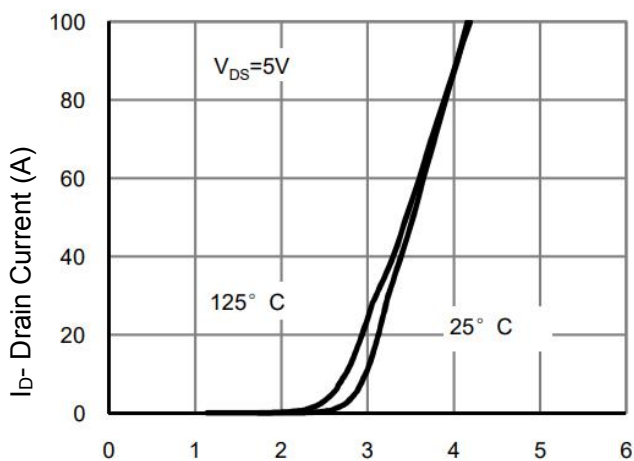
Figure 7 Transfer Characteristics
