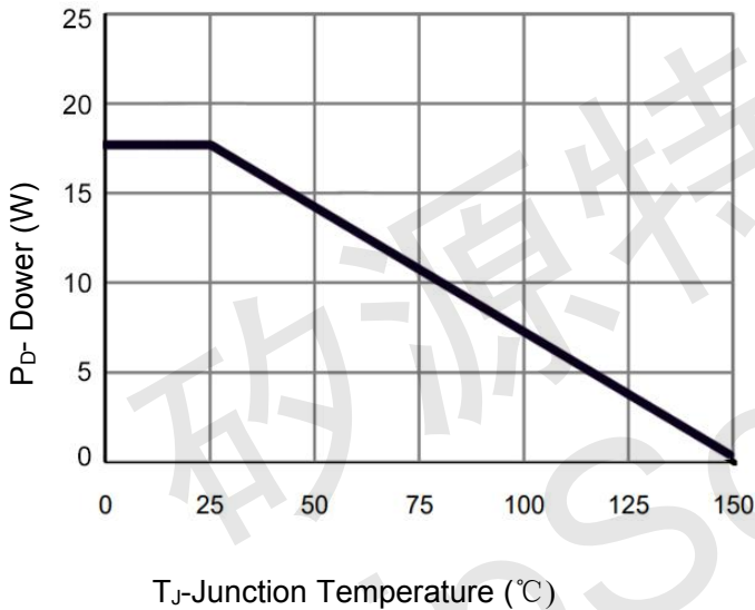
Figure 3 Power De-rating
