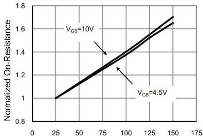
TJ-Junction Temperature(°C) Figure 8 Rdson vs Junction Temperature
