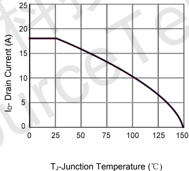
Figure 4 Drain Current
