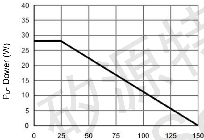
Figure 3 Power De-rating
