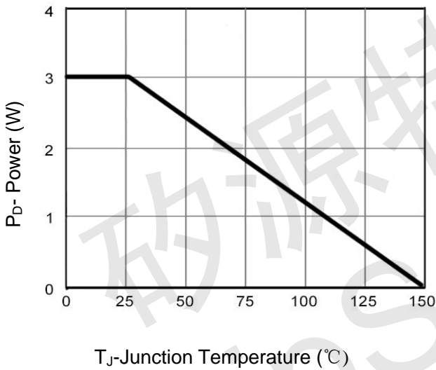
Figure 3 Power De-rating
