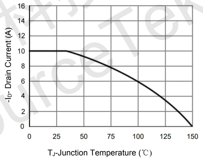
Figure 4 Drain Current
