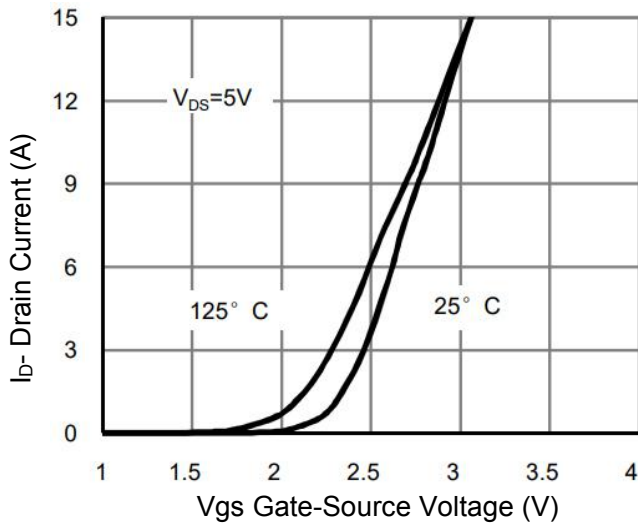
Figure 7 Transfer Characteristics
