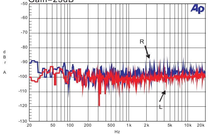
Noise Floor FFT Inputs ac-ground, V_{DD}=5\text{V} , C_{IN}=1\mu\text{F} , R_L=4\Omega , Gain=23dB
