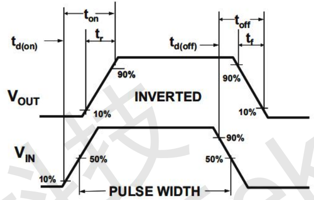
Figure 2: Switching Waveforms
