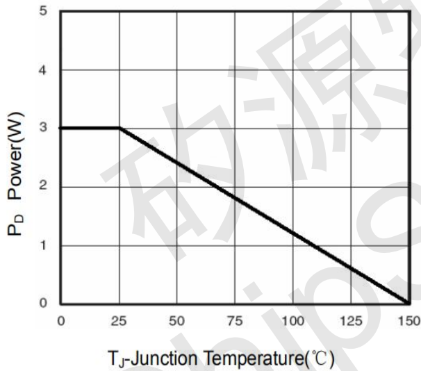
Figure 3 Power Dissipation
