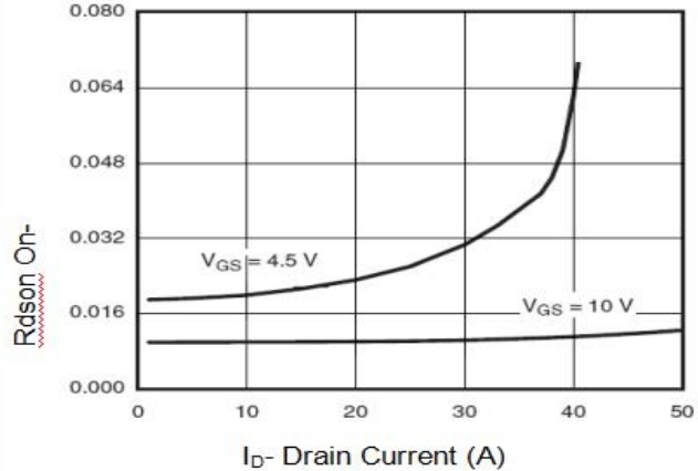
Figure 6 Drain-Source On-Resistance
