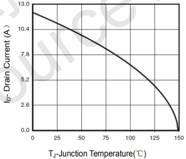
Figure 4 Drain Current
