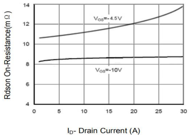
Figure 6 Drain-Source On-Resistance
