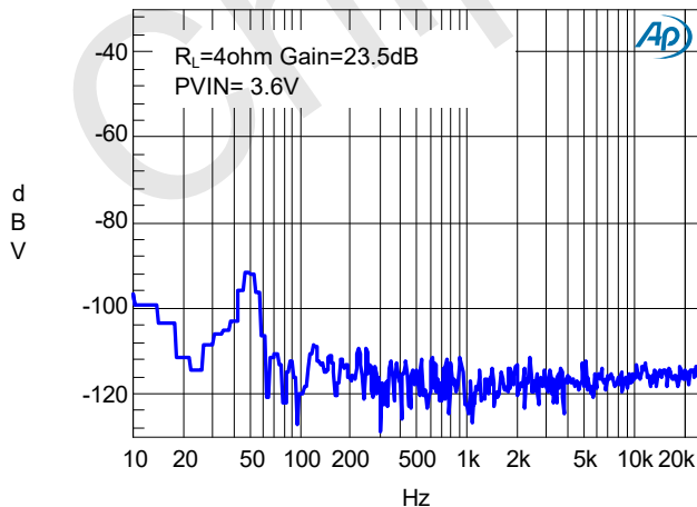
Noise Floor
