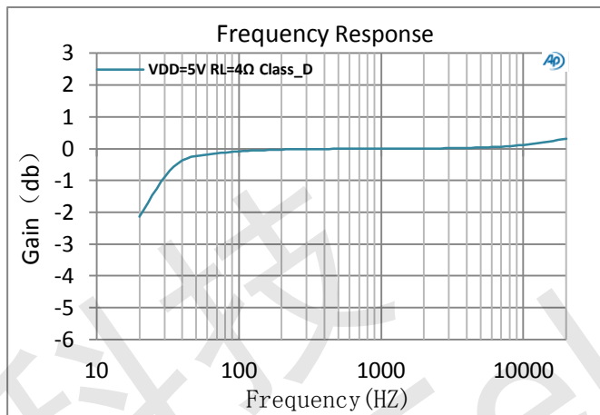
图8: Frequency Response
