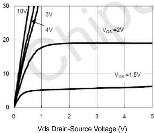
Figure 5 Output CHARACTERISTICS
