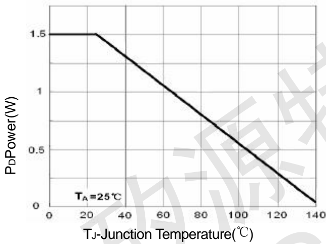
Figure 3 Power Dissipation
