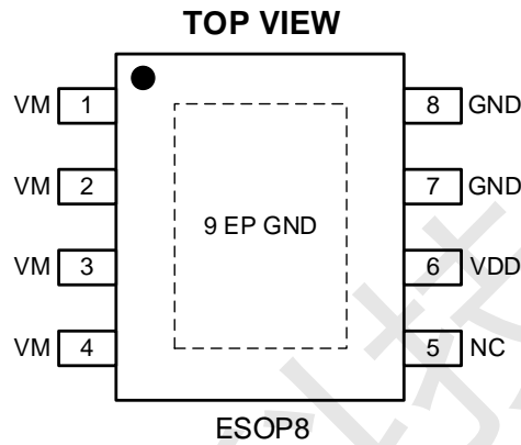
Figure 2. Pin Configuration
