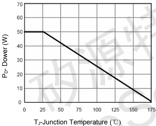
Figure 3 Power De-rating
