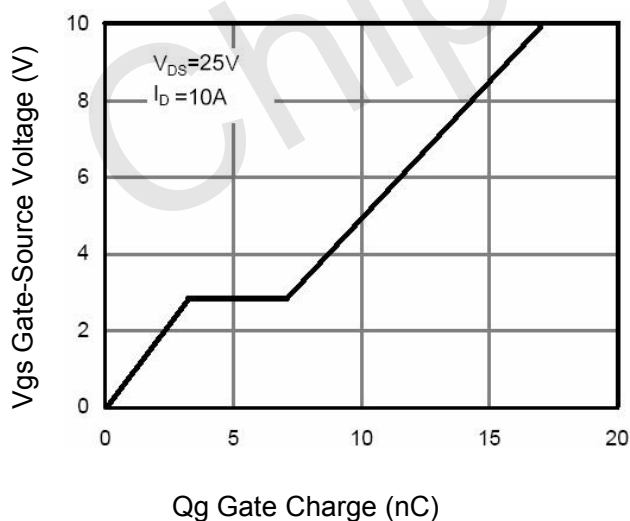
Figure 11 Gate Charge
