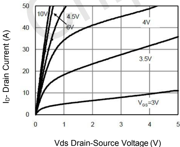
Figure 5 Output Characteristics
