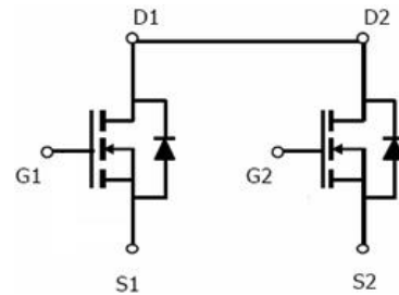
Schematic diagram
