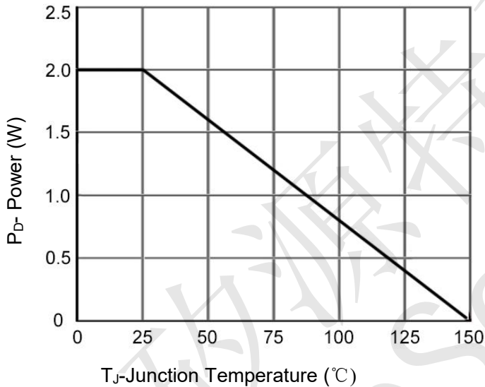
Figure 3 Power De-rating
