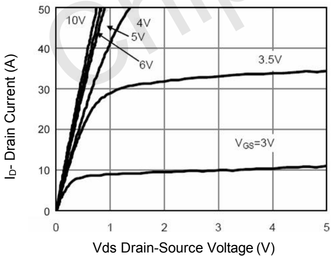
Figure 5 Output Characteristics
