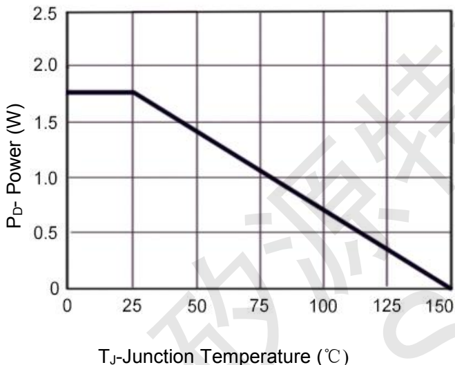
Figure 3 Power De-rating
