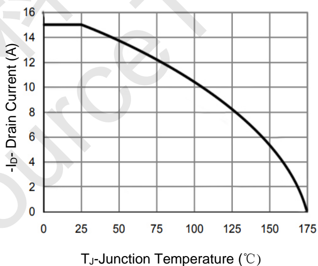
Figure 4 Drain Current
