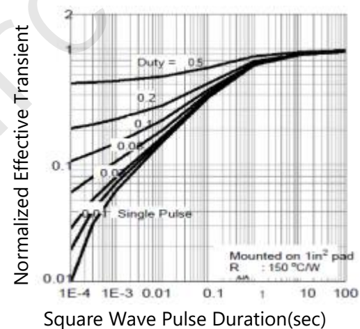
Figure 4. Transient Thermal Impedance
