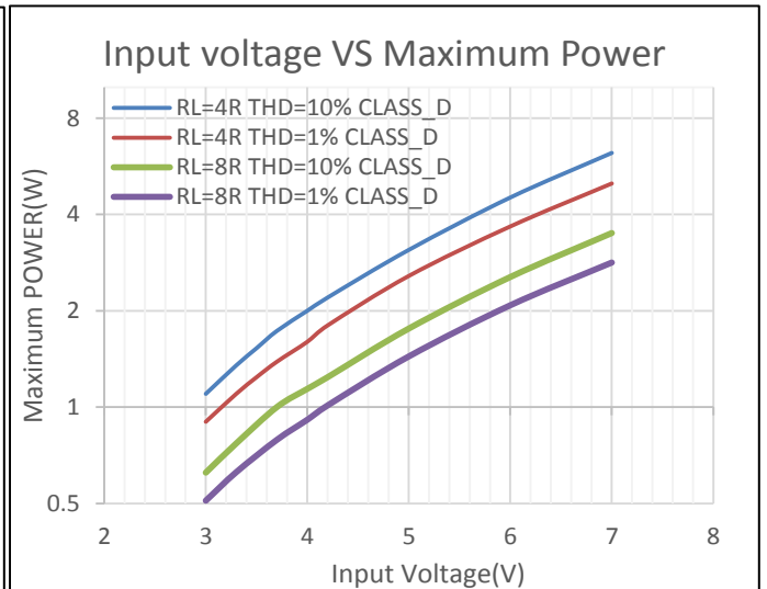
4、Input voltage VS Maximum Power
