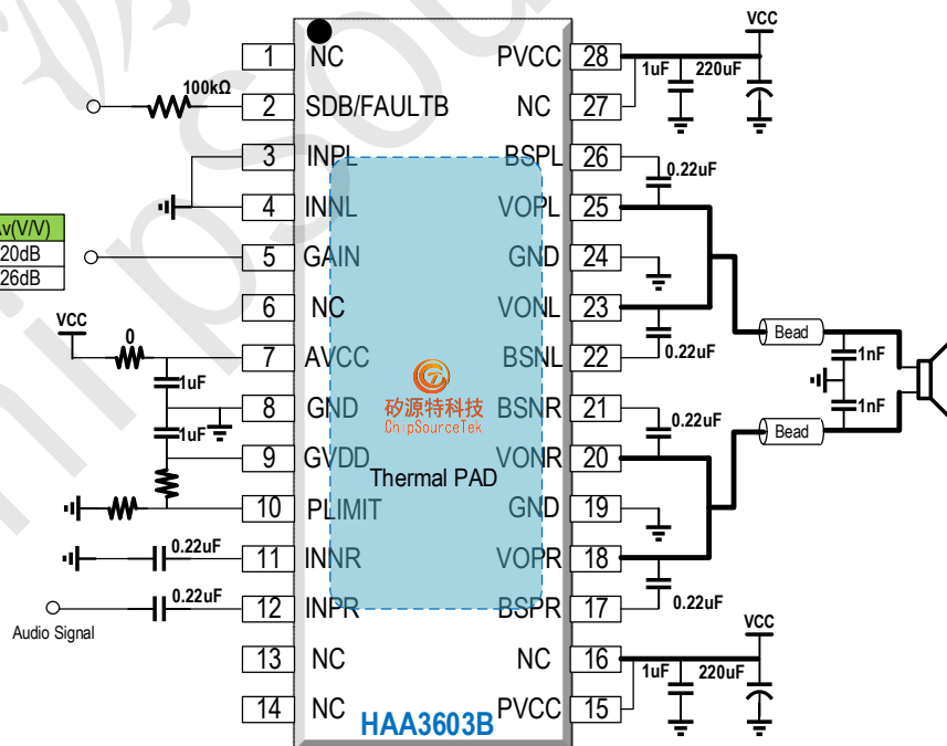
PBTL Configuration with Single-Ended Inputs
