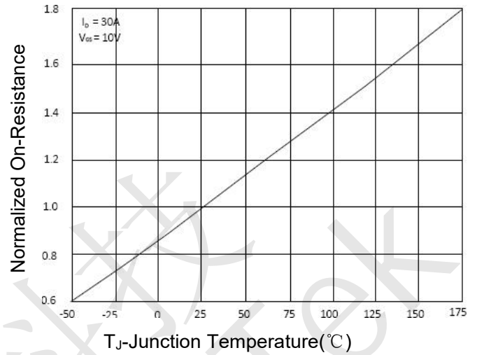
Figure 4 Rdson-Junction Temperature
