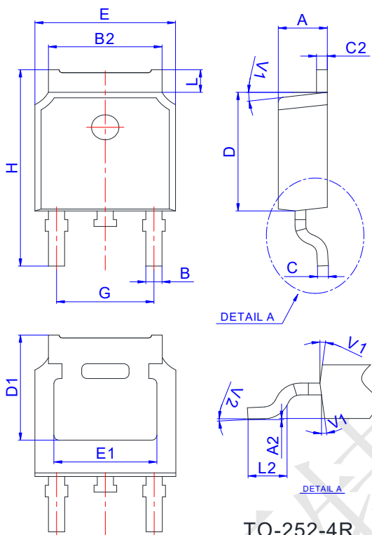
TO-252-4R
