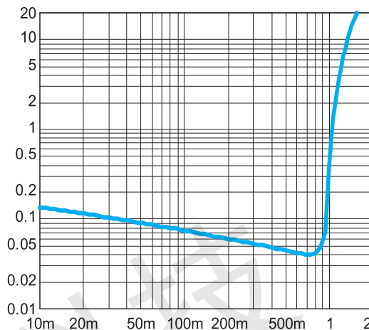
Figure 34. THD+N vs. Output Power BTL mode, 3V, 40hm, f=1 kHz
