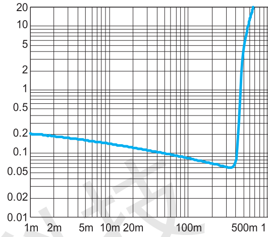
Figure 4. THD+N vs. Output Power 3V, 80ohm, BTL at f=1 kHz
