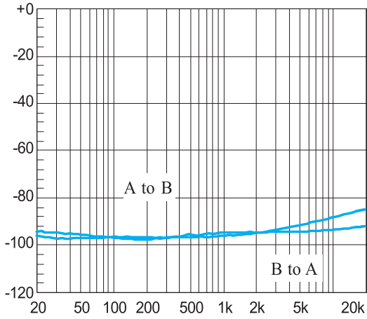
Figure 39. Crosstalk BTL mode, 6V, 8Ohm, Po=1W
