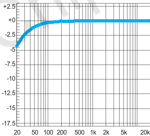
Figure 25. Frequency Response SE mode, 6V, 32Ohm, C5/C6=220uF
