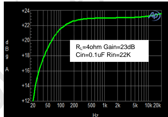
Frequency Response
